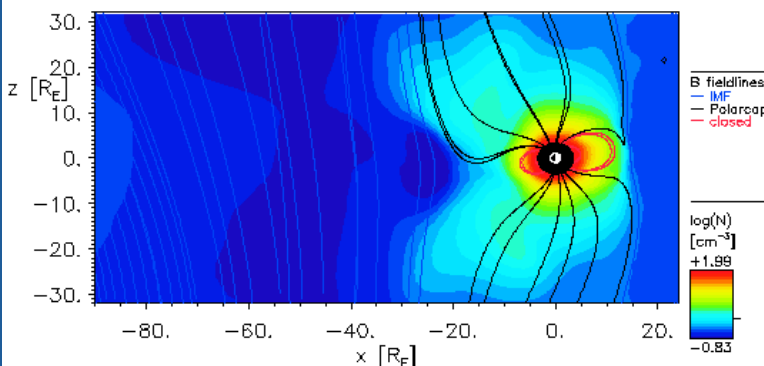
Model at CCMC: BATSRUS
