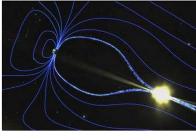
A spacequake in action is seen in this still from an animation of the interaction with Earth's magnetic field. CREDIT: Walt Feimer of Goddard's Scientific Visualization Lab. \
