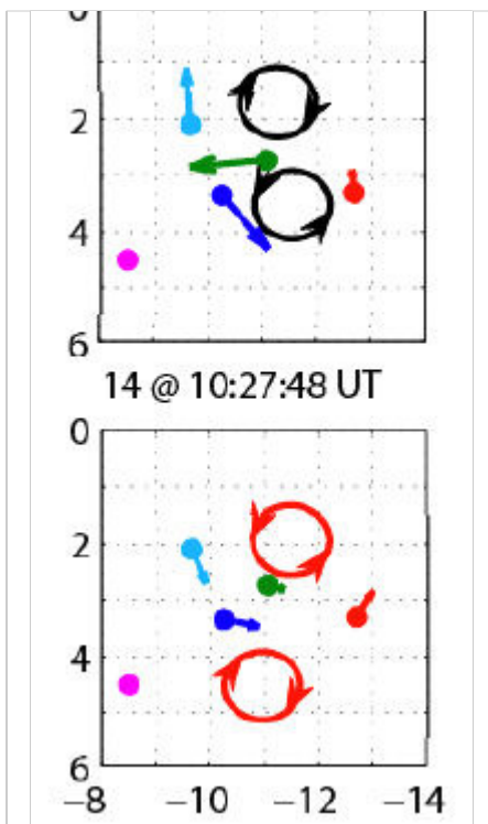
A THEMIS map of plasma flows during a spacequake. The axes are labeled in Earth radii, so each swirl is about the size of Earth. [larger image]
