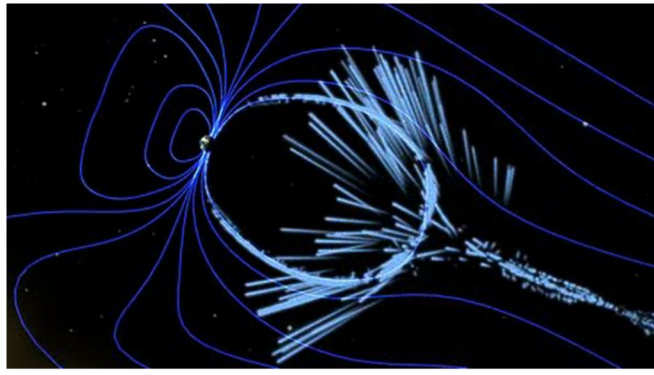
A still from a NASA animation shows a broken magnetic field line triggering a "spacequake."
